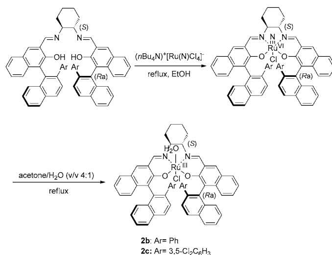
Scheme 4. Preparation of complexes 2b and 2c .
